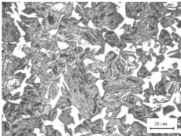
Fig. 4. Microstructure of steel pre-etched with 4% picral.
