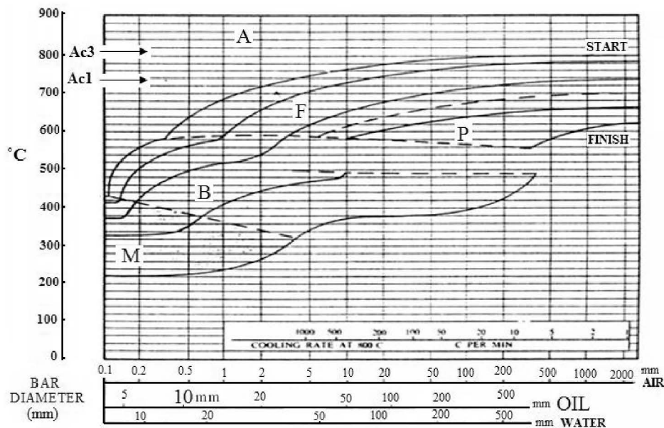
Fig. 1. The CCT diagram of DIN 1.6526 steel 6) .
