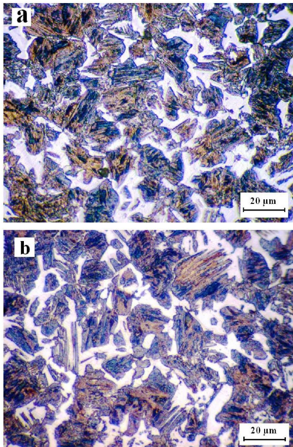
Fig. 6. Micrographs of the specimen resulted from technique (3).
