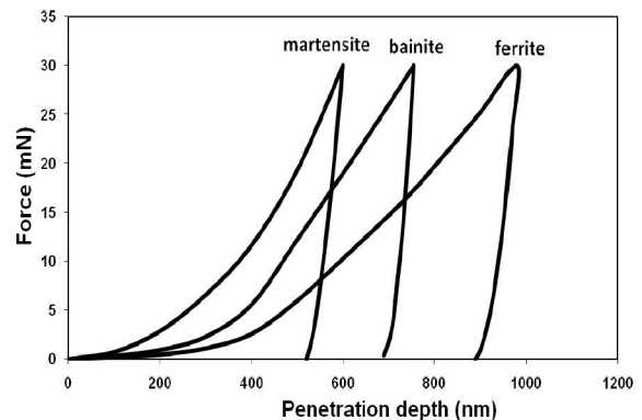
Fig. 7. The force versus penetration depth for different phases in the nanoindentation test.
