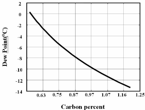
Fig. 3. Dewpoint vs. surface carbon percent at 927 °C, 1 atmosphere, and 2.51- 2.6 air/fuel ratio.
