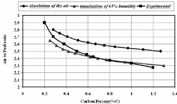
Fig. 9 Variations in carbon percent with changes in air/fuel ratio under experimental and simulated conditions for dry and wet air at 880 °C, 1 atmosphere, ambient temperature of 21 °C, and relative humidity of 65%.
